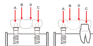
A. Fracture on the implant side B. Fracture between pontic and implant C. Fracture on the tooth side D. Fracture between pontic and tooth. For the implant-implant situation failure pattern A is equivalent to C and B to D.
